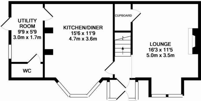
GROUND FLOOR APPROX. FLOOR AREA 460 SQ.FT. (42.7 SQ.M.)
